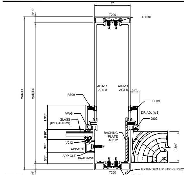
D STRIKE JAMB & S.L. MULLION W/ 2" FACE
