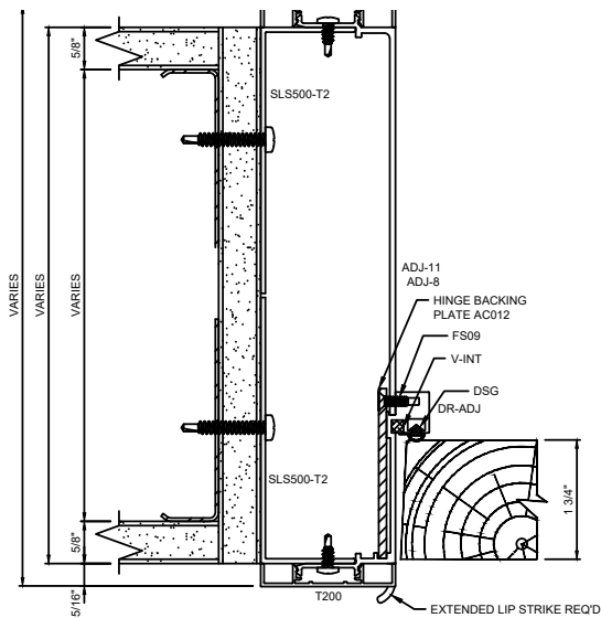
N DOOR FRAME STRIKE JAMB W/ STARTER TRACK
