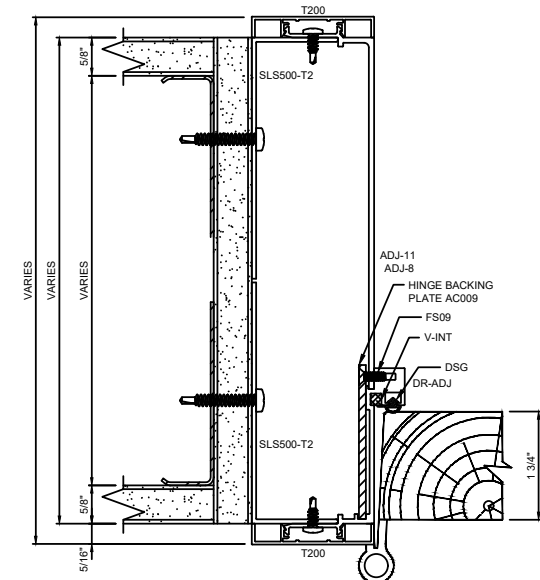
M DOOR FRAME HINGE JAMB W/ STARTER TRACK
