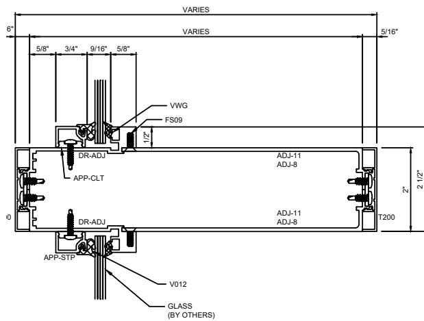
G HORIZONTAL MULLION W/ 2" FACE
