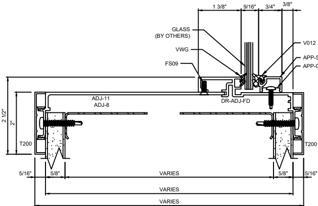
E SILL BASE ON DRYWALL PARTITION
