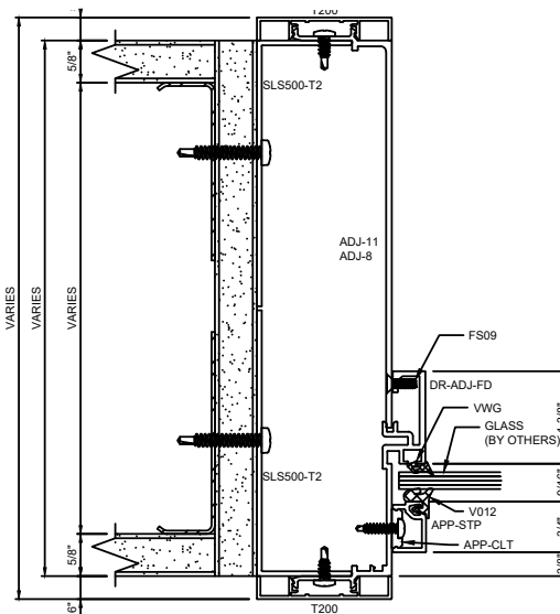
O GLAZING JAMB W/ STARTER TRACK
