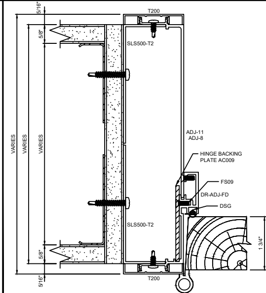
M DOOR FRAME HINGE JAMB W/ STARTER TRACK
