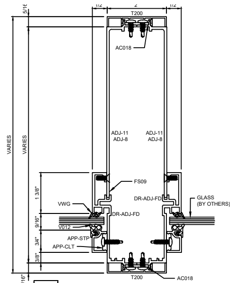
H VERTICAL MULLION W/ 2" FACE
