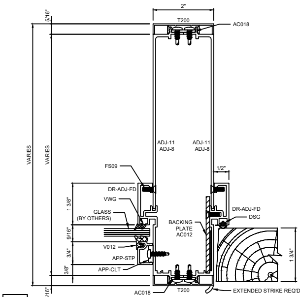
D STRIKE JAMB & S.L. MULLION W/ 2" FACE
