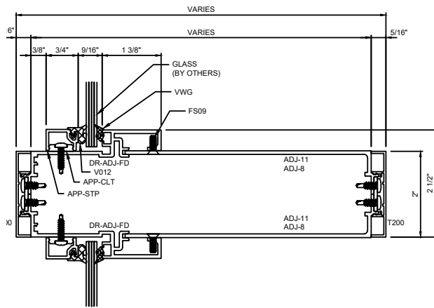
G HORIZONTAL MULLION W/ 2" FACE
