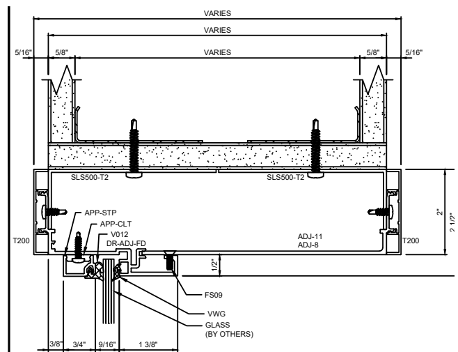
P HEAD MULLION W/ STARTER TRACK
