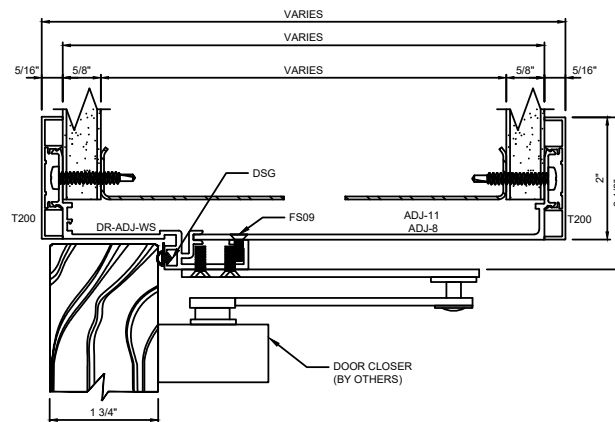
L DOOR HEADER WITH WIDE STOP FOR CLOSER ARM ATTACHMENT
