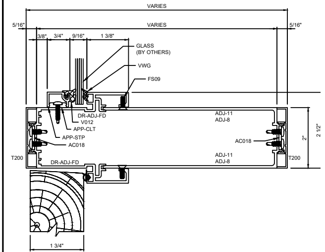
I TRANSOM HEADER W/ 2" FACE
