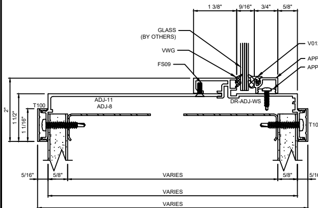
E SILL BASE ON DRYWALL PARTITION
