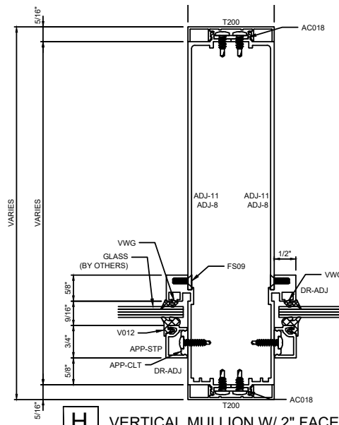
H VERTICAL MULLION W/ 2" FACE
