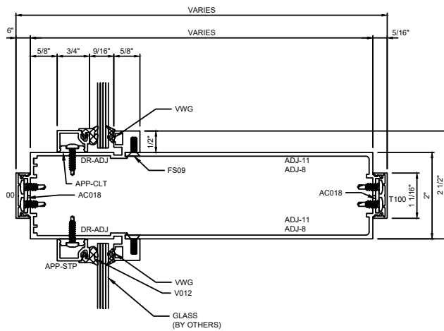
G HORIZONTAL MULLION W/ 2" FACE
