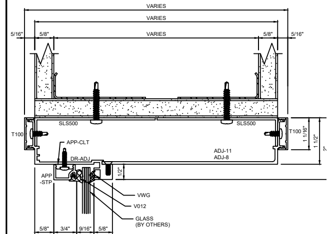
P HEAD MULLION W/ STARTER TRACK
