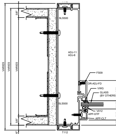
O GLAZING JAMB W/ STARTER TRACK
