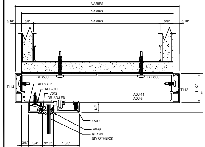
P HEAD MULLION W/ STARTER TRACK
