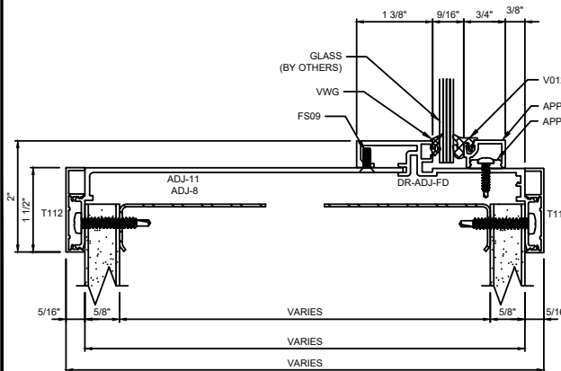
E SILL BASE ON DRYWALL PARTITION
