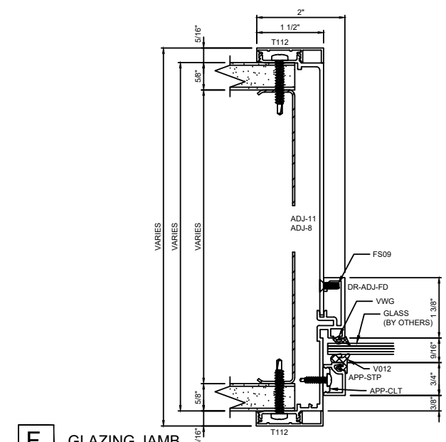
F GLAZING JAMB
