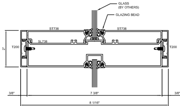
G HORIZONTAL MULLION W/ 2" FACE
