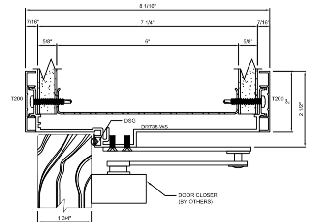
I OPTIONAL HEADER: WIDE STOP FOR SURFACE CLOSER ATTACHMENT
