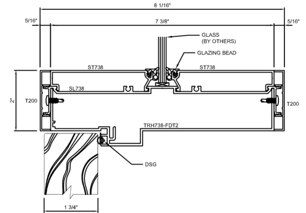
I TRANSOM HEADER W/ 2" FACE
