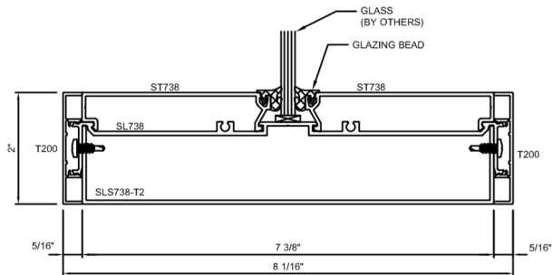
J GLAZING SILL W/ STARTER TRACK
