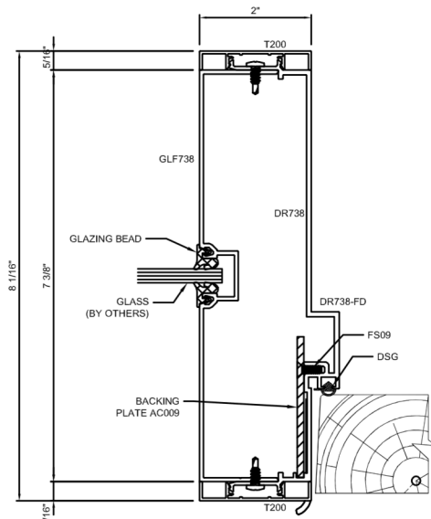
D STRIKE JAMB & S.L. MULLION W/ 2" FACE
