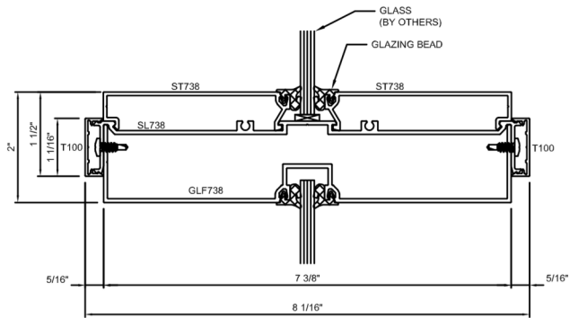
G HORIZONTAL MULLION W/ 2" FACE
