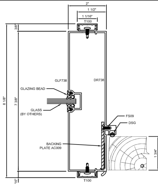
D STRIKE JAMB & S.L. MULLION W/ 2" FACE
