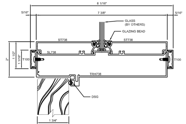
I TRANSOM HEADER W/ 2" FACE
