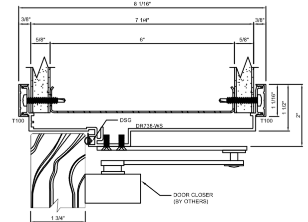
L OPTIONAL HEADER: WIDE STOP FOR SURFACE CLOSER ATTACHMENT
