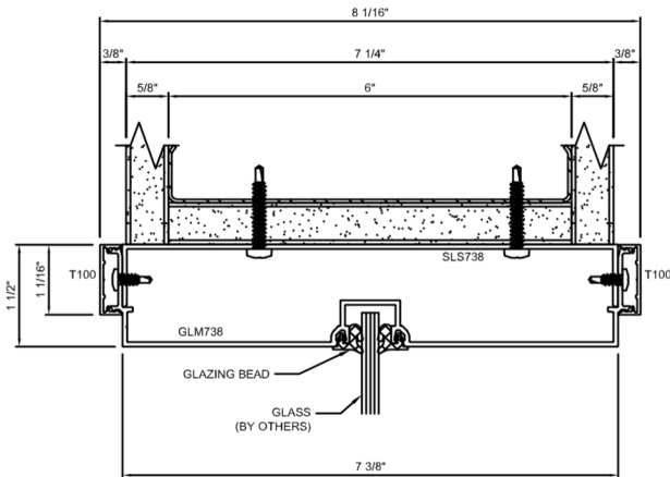
P HEAD MULLION W/ STARTER TRACK
