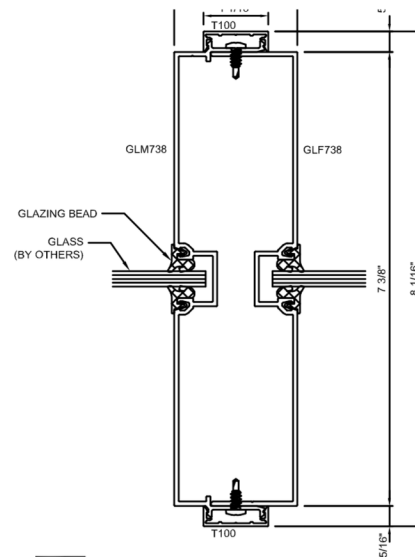
H VERTICAL MULLION W/ 2" FACE
