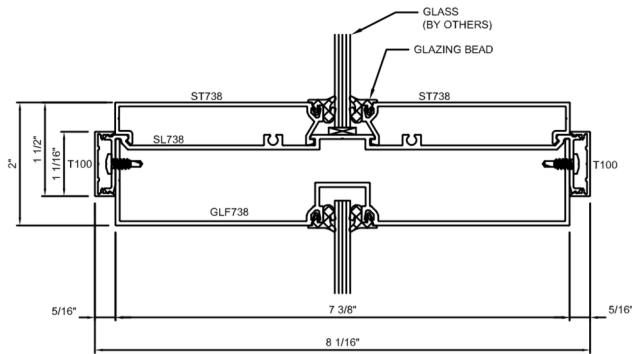
G HORIZONTAL MULLION W/ 2" FACE
