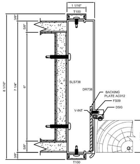
N DOOR FRAME STRIKE JAMB W/ STARTER TRACK
