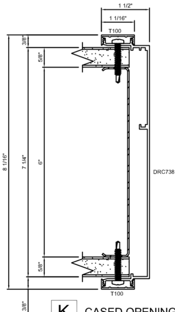
K CASED OPENING
