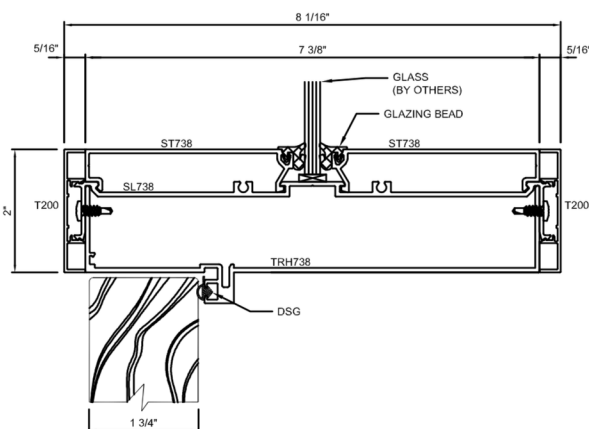
Q TRANSOM HEADER W/ 2" FACE
