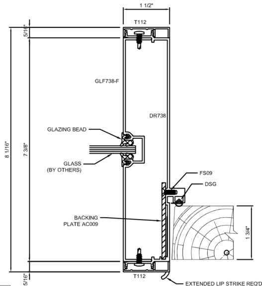
D STRIKE JAMB & S.L. MULLION W/ 1-1/2" FACE
