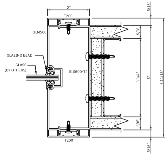
O GLAZING JAMB W/ STARTER TRACK
