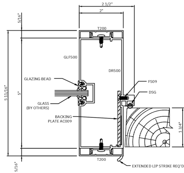
D STRIKE JAMB & S.L. MULLION W/ 2" FACE
