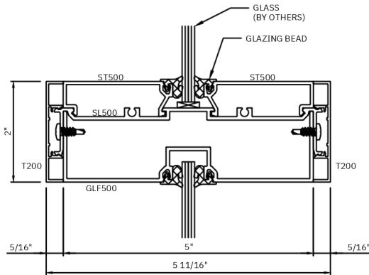
G HORIZONTAL MULLION W/ 2" FACE
