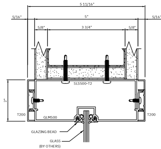
P HEAD MULLION W/ STARTER TRACK
