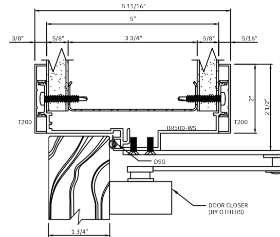
L DOOR HEADER WITH WIDE STOP FOR CLOSER ARM ATTACHMENT
