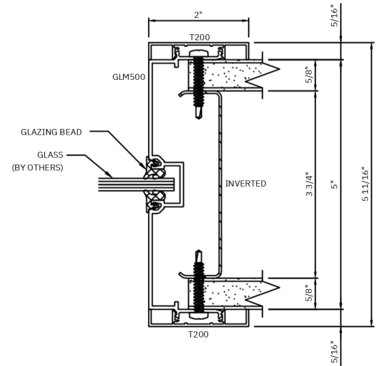
F GLAZING JAMB
