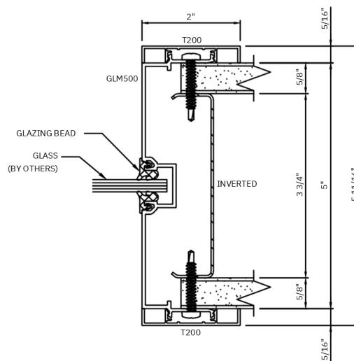
F GLAZING JAMB
