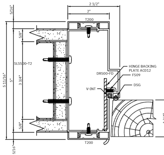
N DOOR FRAME STRIKE JAMB W/ STARTER TRACK
