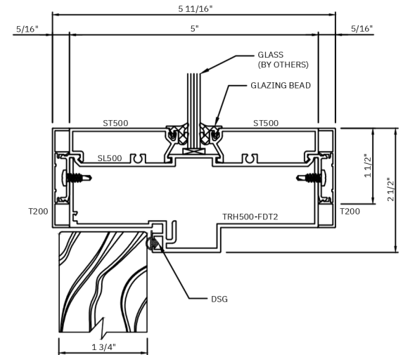
I TRANSOM HEADER W/ 2" FACE
