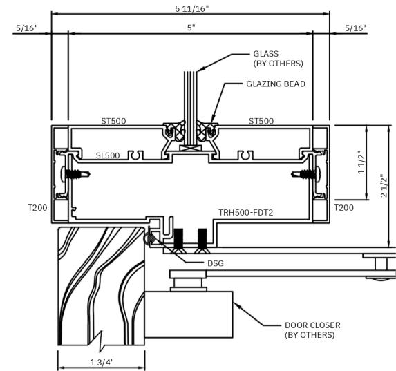
L DOOR HEADER WITH WIDE STOP FOR CLOSER ARM ATTACHMENT
