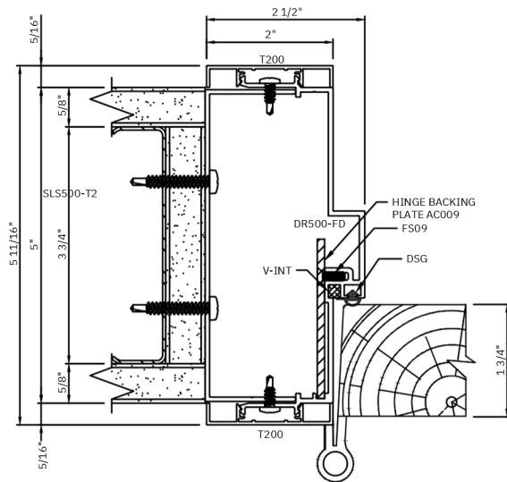
M DOOR FRAME HINGE JAMB W/ STARTER TRACK
