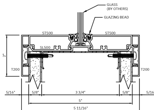
E SILL BASE ON DRYWALL PARTITION
