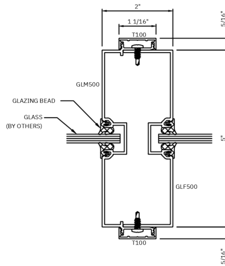
H VERTICAL MULLION W/ 2" FACE
