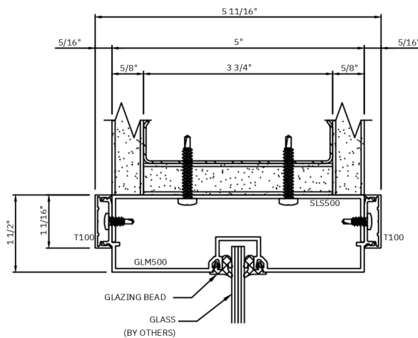
P HEAD MULLION W/ STARTER TRACK
