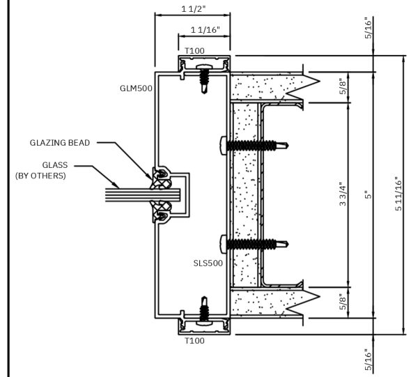
O GLAZING JAMB W/ STARTER TRACK
