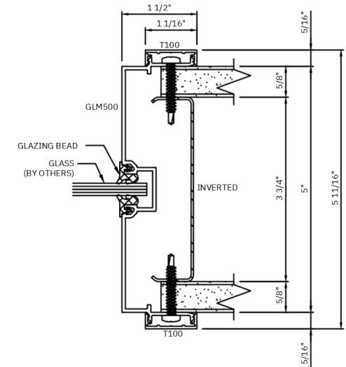
F GLAZING JAMB
