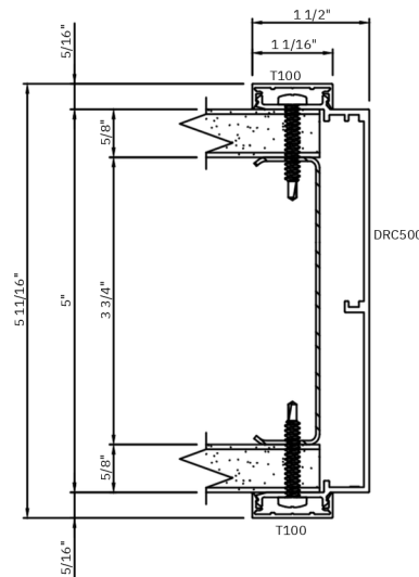
K CASD OPENING
