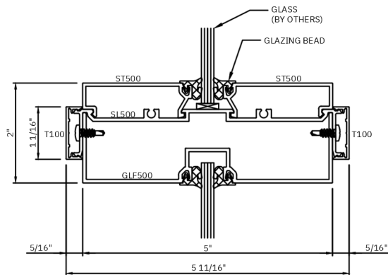
G HORIZONTAL MULLION W/ 2" FACE
