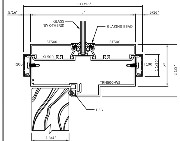
I TRANSOM HEADER W/ 2" FACE
