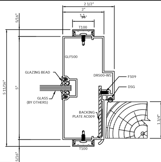
D STRIKE JAMB & S.L. MULLION W/ 2" FACE
