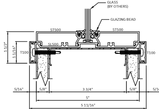
E SILL BASE ON DRYWALL PARTITION
