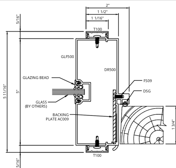
D STRIKE JAMB & S.L. MULLION W/ 2" FACE
