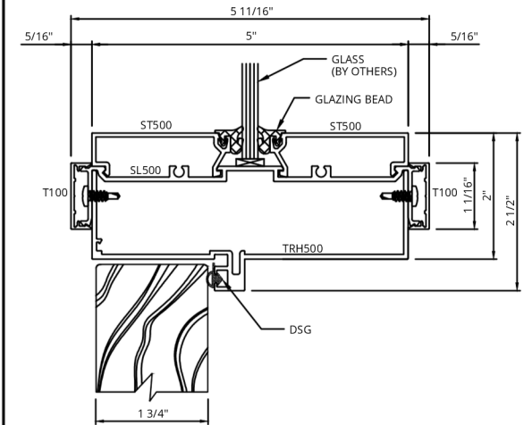
I TRANSOM HEADER W/ 2" FACE
