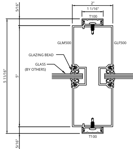
H VERTICAL MULLION W/ 2" FACE
