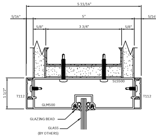
P HEAD MULLION W/ STARTER TRACK
