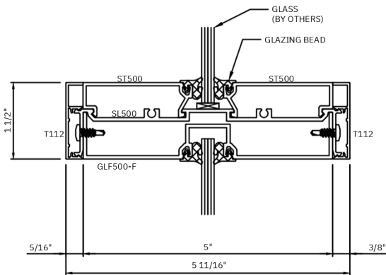
G HORIZONTAL MULLION W/ 1-1/2" FACE
