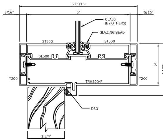
Q TRANSOM HEADER W/ 2" FACE
